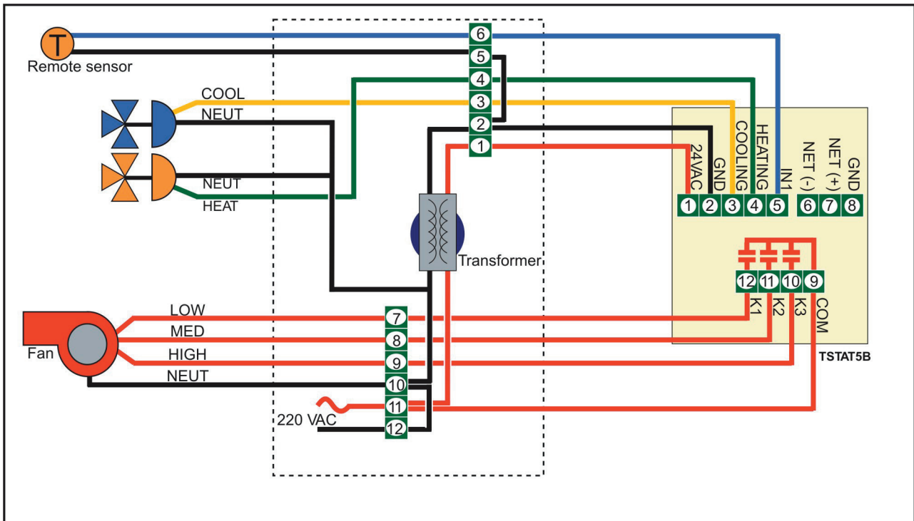
Tstat5B - 220VAC ON/OFF Valves, 3-Speed Fan
