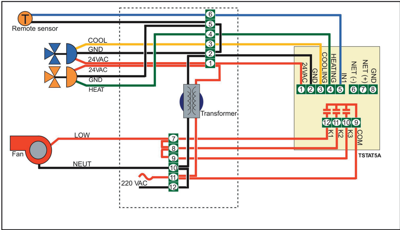
Tstat5A - 24VAC Modulating Valves, 1-Speed Fan
